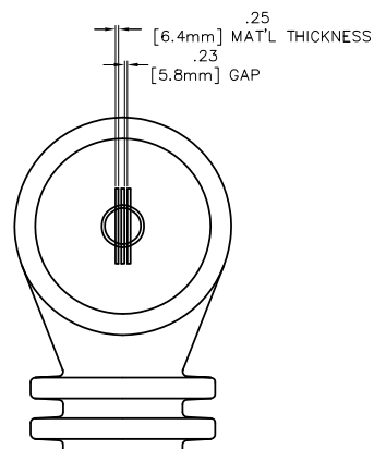
PAD CONFIGURATION FOR 3000:5 3 PADS EACH SIDE
